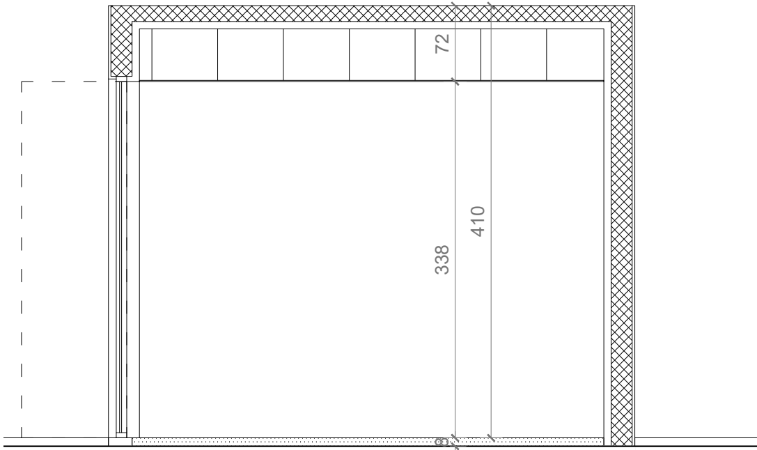
Section 2-2
